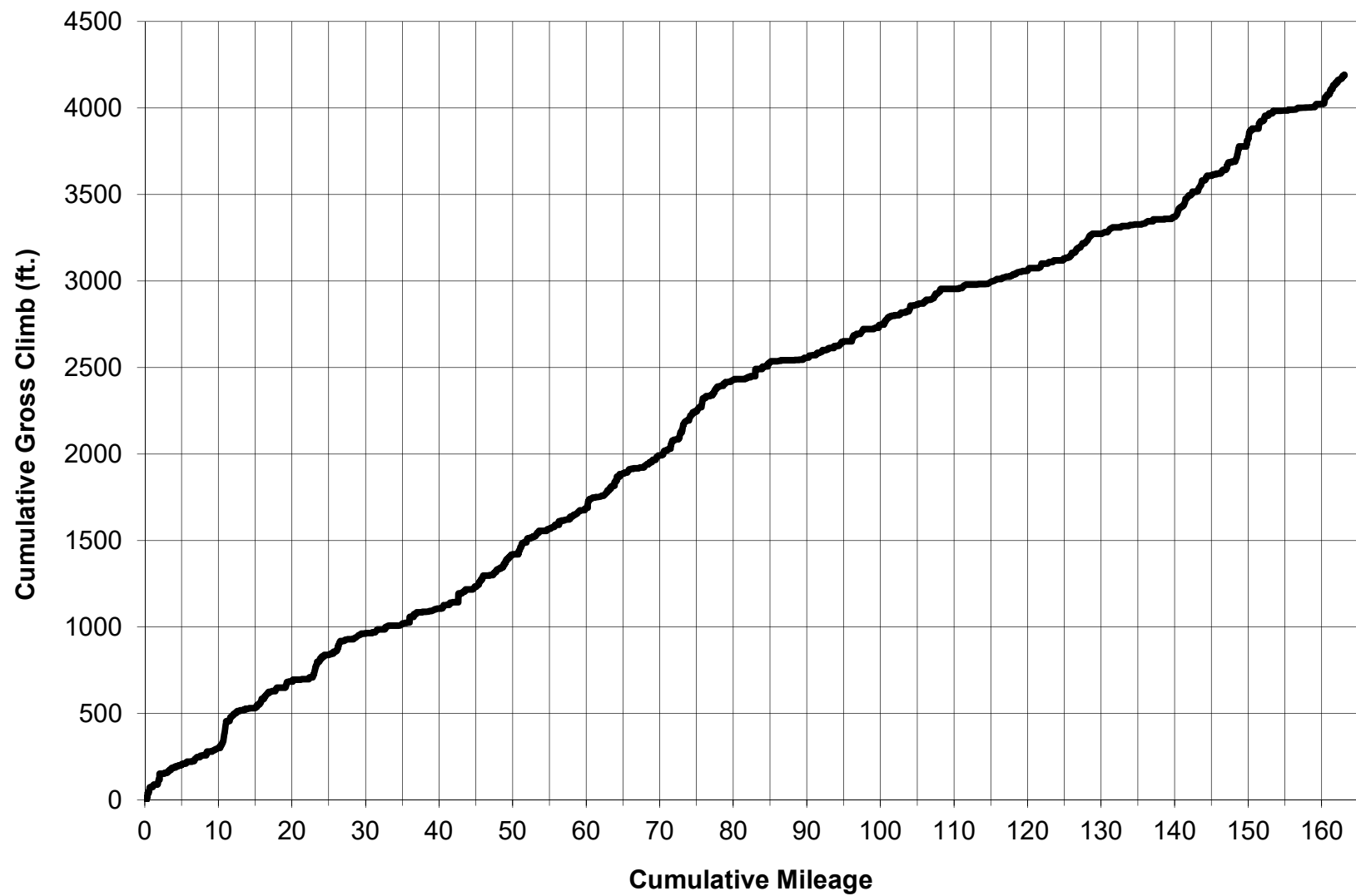
RAIL South Gross Climb Profile - St. Louis, MO to Vincennes, IN
