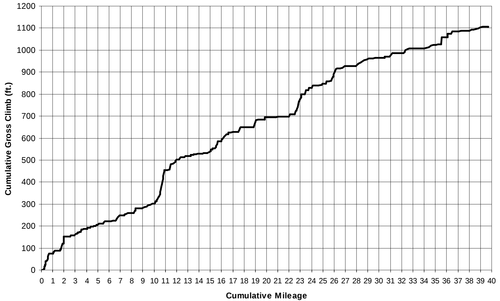
RAIL South Ride 1 Gross Climb Profile - St. Louis to Breese
