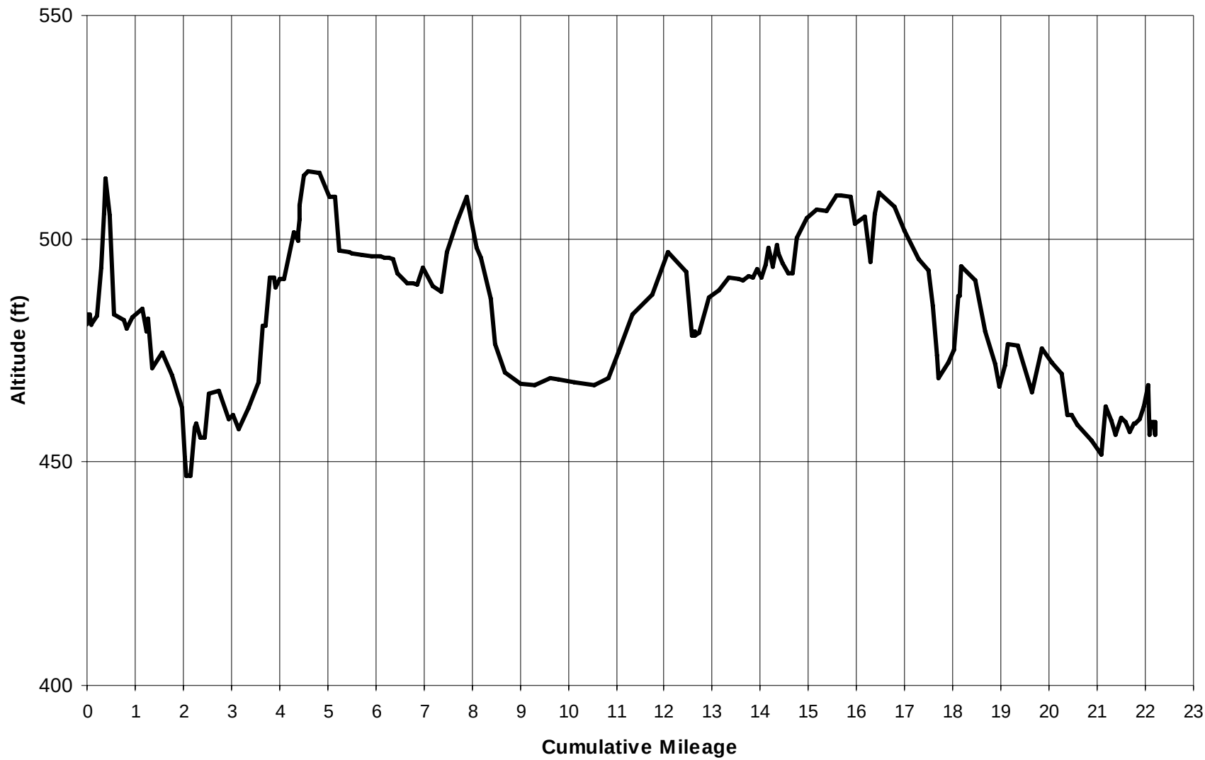
RAIL South Ride 4 Elevation Profile - Flora to Olney
